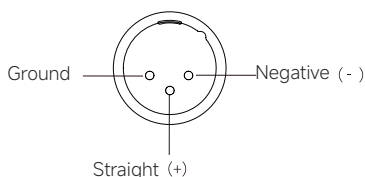
Set reverse port polarity diagram
