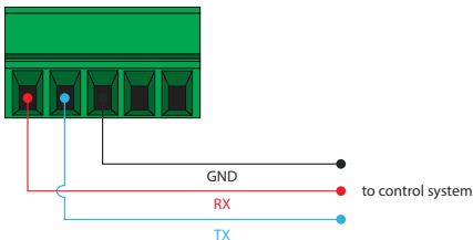
Figure 1.1 - Wiring the 5-pin HDBaseT RS-232/IR captive screw block for RS-232 control of a source device connected to headend matrix.
